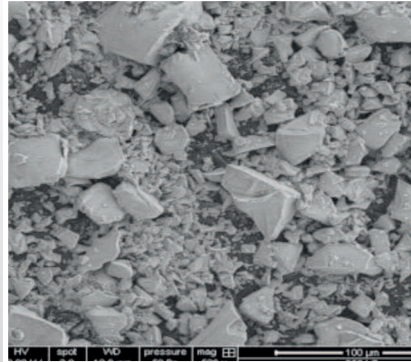
The coating on Thermiculite® 866 prior to use
